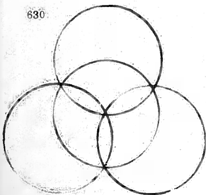
O'Beirne's four-circle problem
