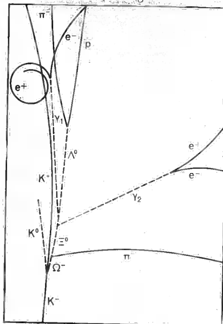
Diagram of production of omega minus (left) and map of events
