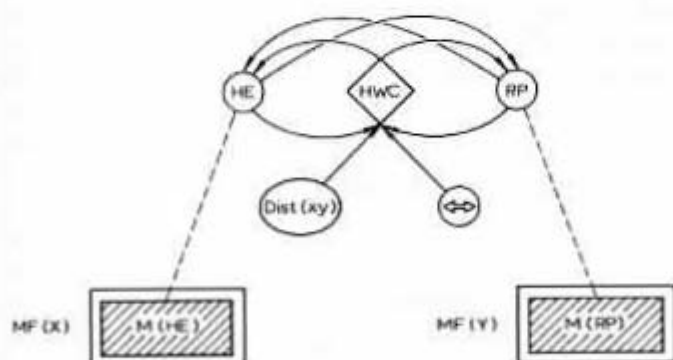
Fig. 7.2. Proposed (and limited) isomorphic analogy between "Heat Engine" (HE) and "Refrigerator Heat Pump" (RP). Models are constructed in distinct and a-priori-independent modelling facilities, MF(X) and MF(Y) . Isomorphism is shown as the operator \leftrightarrow . Dist(x, y) is the predicate or set of predicates, distinguishing the universes X and Y .
