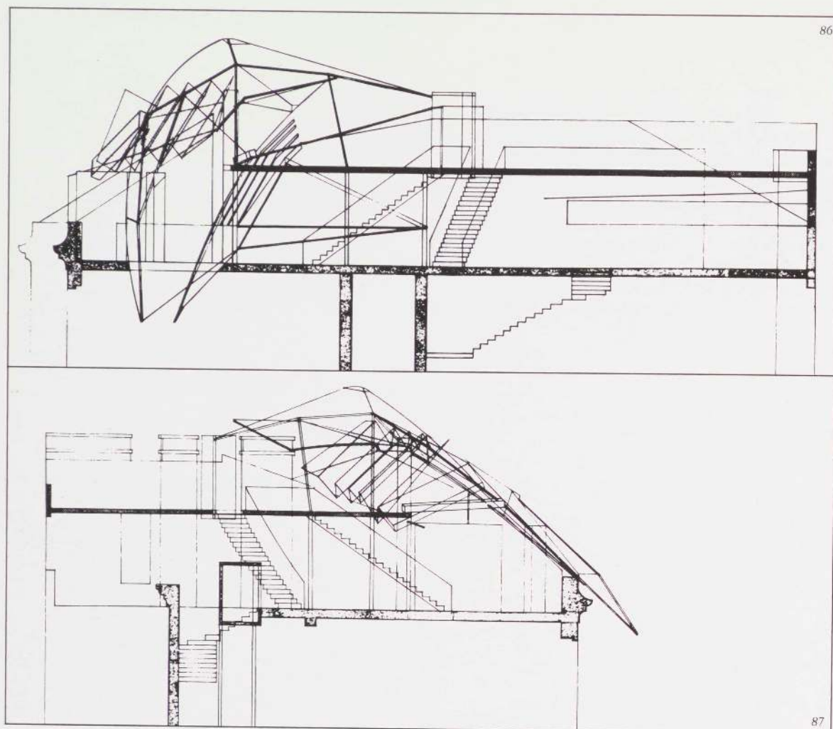
Rooftop Remodeling 85. (Overleaf) Roof plan 86. Longitudinal section 87. Transverse section 88. Structural model 89. Site model
